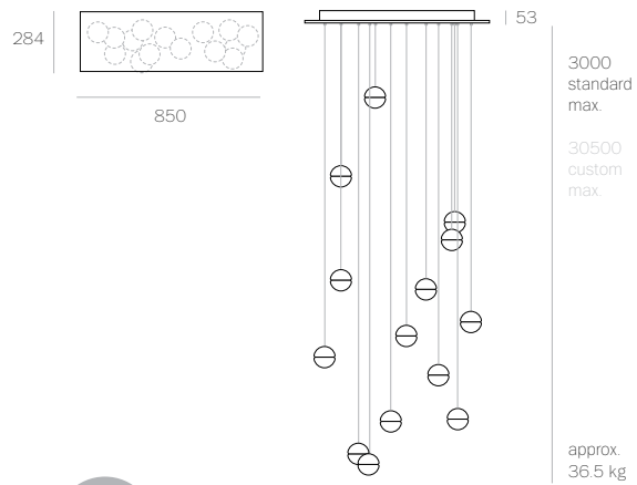
14.14 Rectangle
