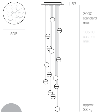
14.14 Round
