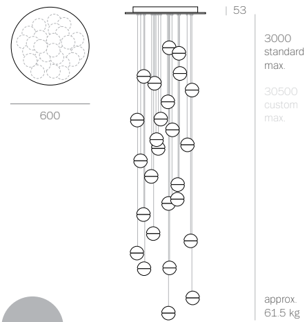
14.26 Round
